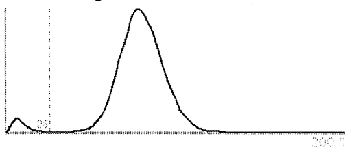
RBC Histogram
