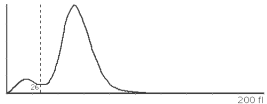
EOS Histogram
