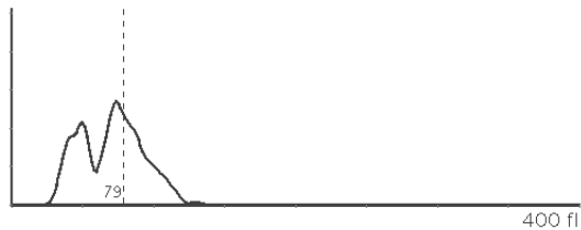
EOS Histogram
