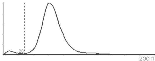
EOS Histogram
